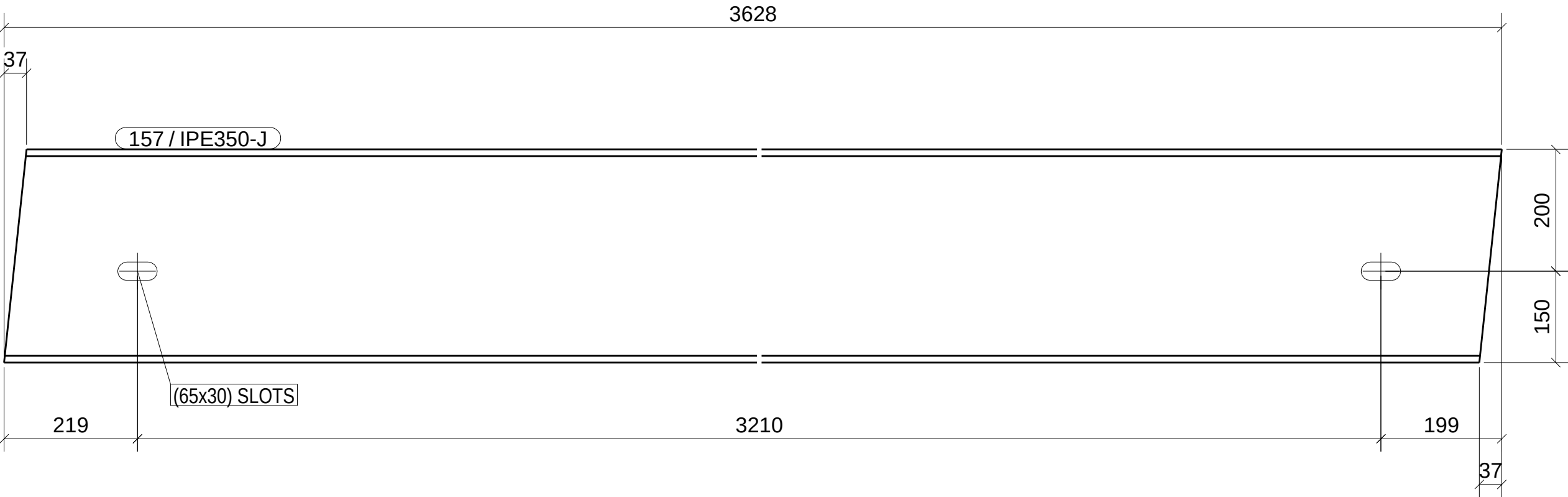
FRONT VIEW
